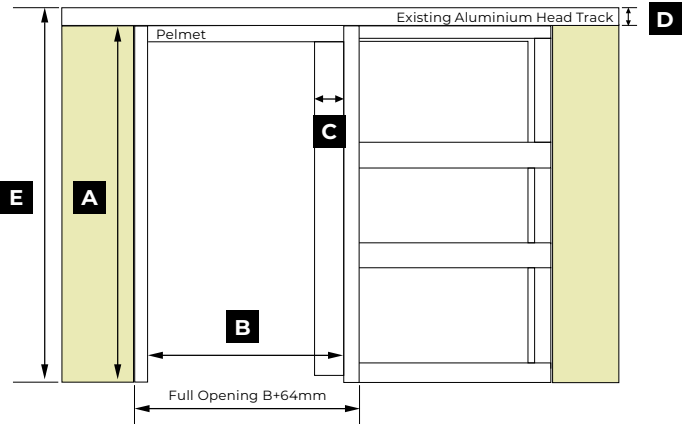
OPTION 1 - Full height into existing aluminium head track
