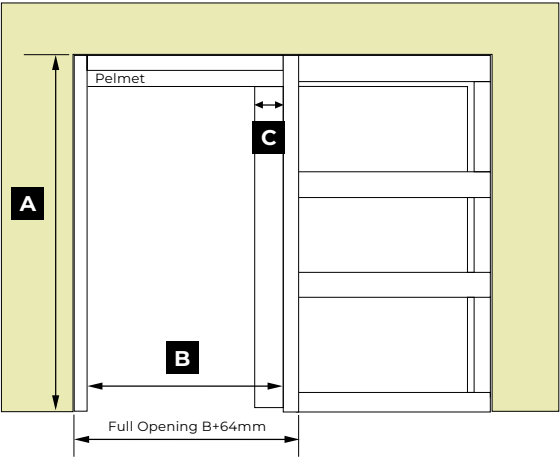
OPTION 3 - Plasterboard above unit
