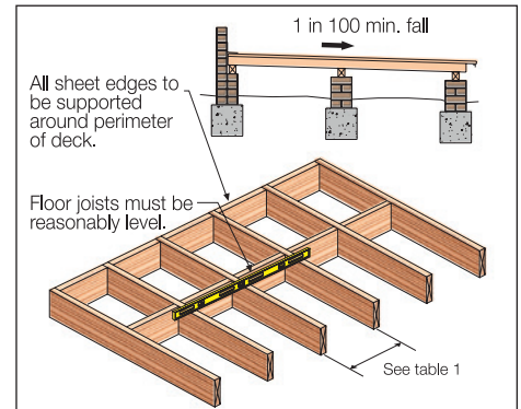
FIGURE 1 FRAME PREPARATION
