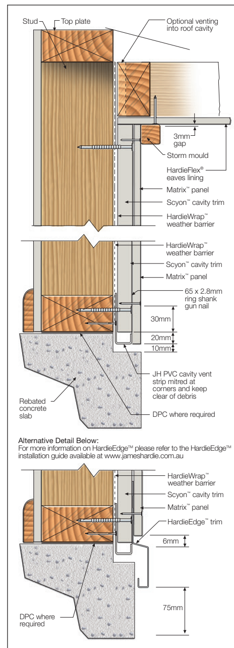
FIGURE 23 SLAB/EAVES DETAIL
