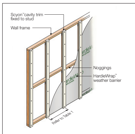
FIGURE 4 ON-STUD FIXING
