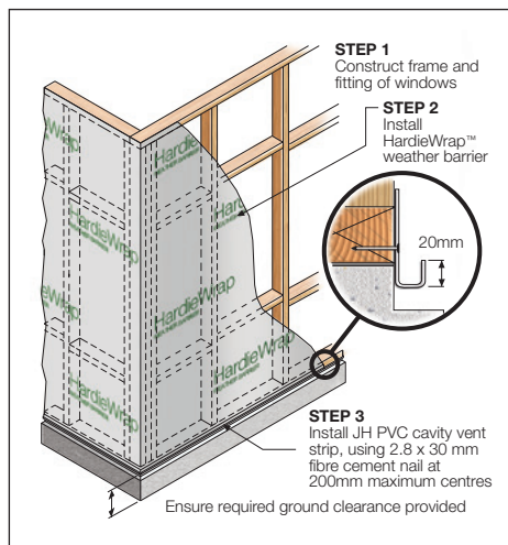
FIGURE 3 PREPARATION
