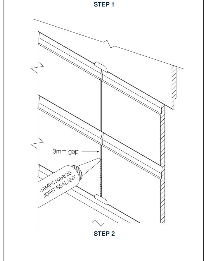
FIGURE 18 UNCLIP ACCESSORY FOR PRIMELINE HERITAGE AND CHAMFER WEATHERBOARDS OFF-STUD JOINTING
