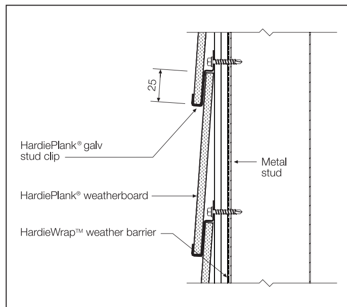
FIGURE 25 FIXING HARDIEPLANK STUD CLIPS
