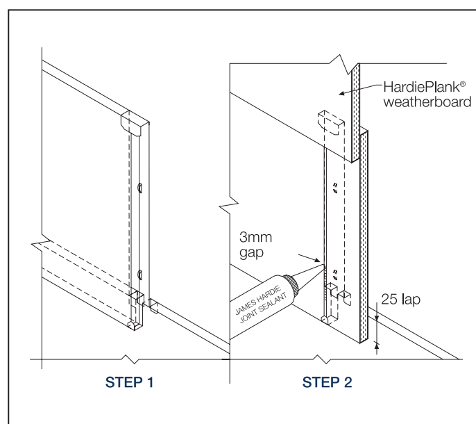
FIGURE 26 FITTING METAL SOAKER
